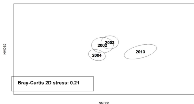
Figure 3. Changes in recruit community structure over the decadal time scale shown by nonmetric multidimensional scaling analysis (NMDS). ANOSIM indicates that changes in recruit densities were significant ( p < 0.05 ).
