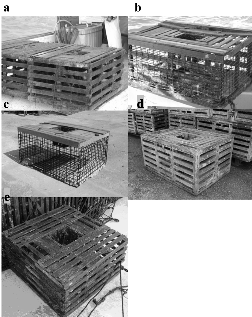
Figure 1. Types of lobster traps used in Florida. a) wood trap, b) wire-reinforced trap, c) wire trap, d) plastic trap, and e) large trap. Large traps are typically 90 cm x 120 cm or 90 cm x 90 cm (as shown). Other traps are typically 60 cm x 80 cm.
