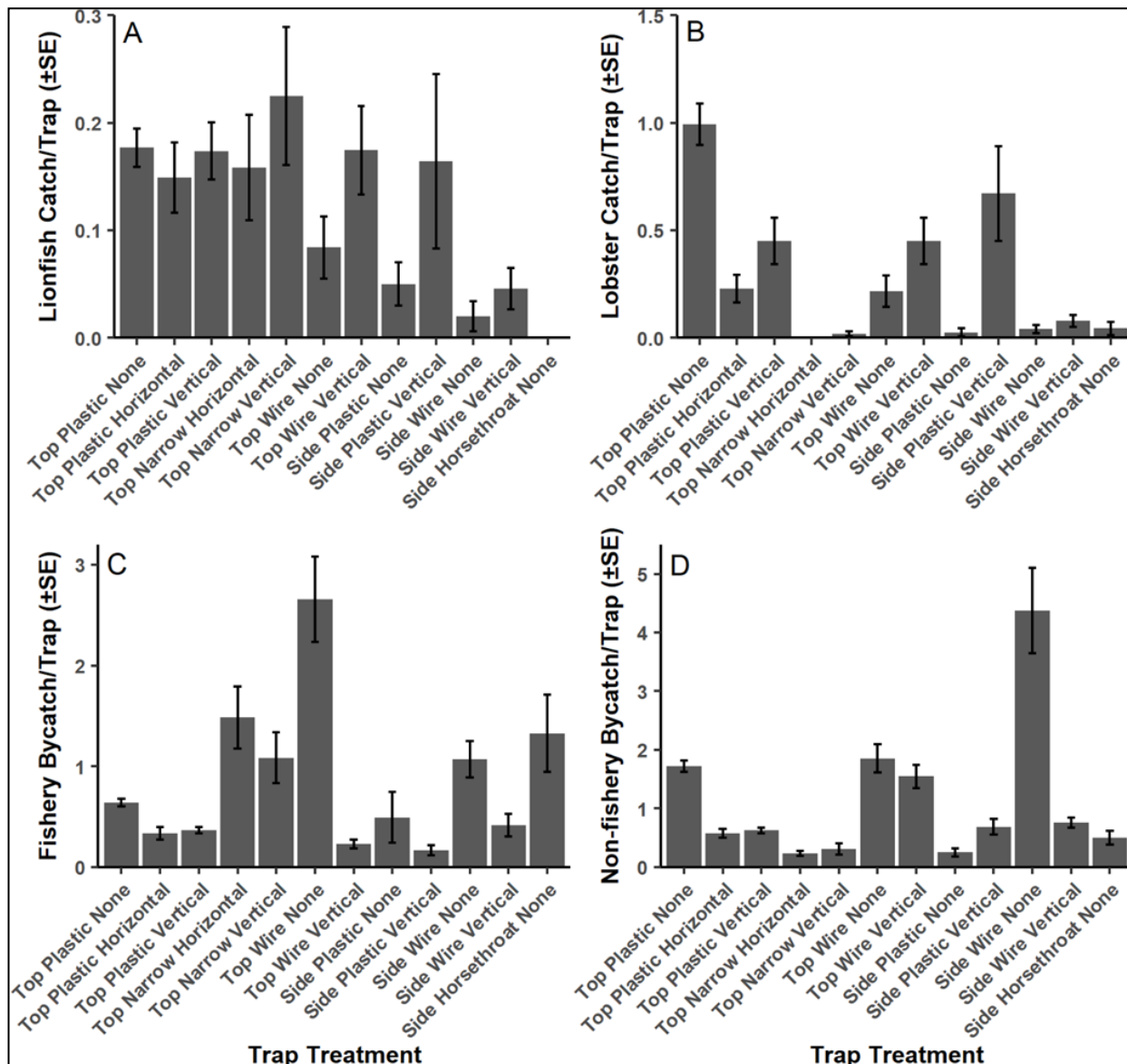
Figure 2. Average catch per trap (±SE) of A) lionfish, B) lobster, C) fishery bycatch, and D) non-fishery bycatch for each trap treatment (all bait types pooled). Trap treatments include throat placement (top or side), throat type (plastic, narrow plastic, wire, or horsethroat), and escape gap type (vertical, horizontal, or none).
