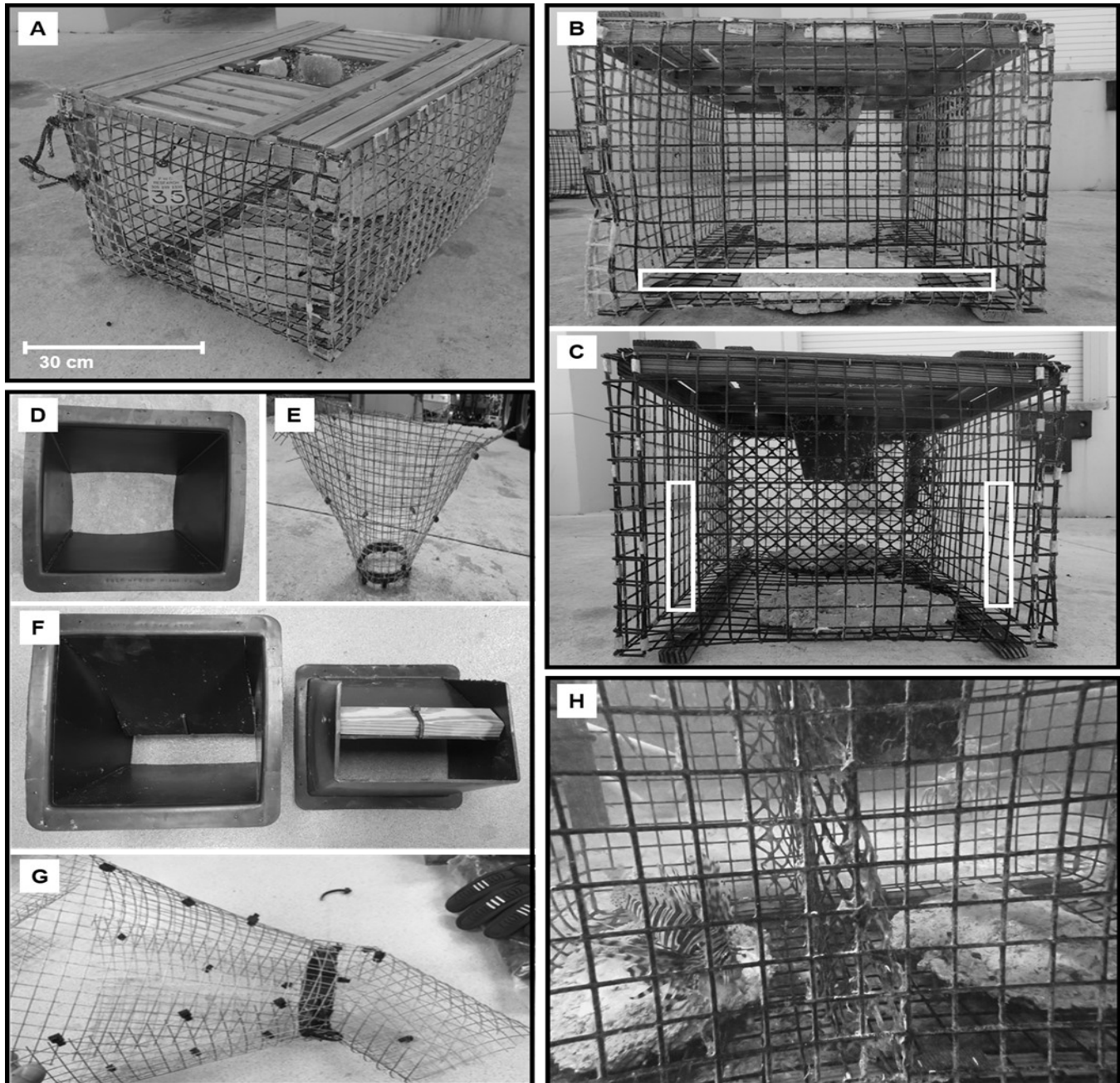
Figure 1. Images of A) a Florida wire spiny lobster trap, B) a horizontal escape gap, C) vertical escape gaps, D) a plastic throat with a 15.2 cm opening, E) a wire throat with a 10.2 cm opening, F) a top and bottom view of a narrow plastic throat with a 5.4 cm opening, G) a wire horsethroat, and H) a trap with a lionfish enclosure and live lionfish bait. The white rectangles in images B and C indicate the escape gaps.
